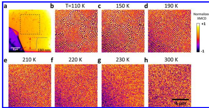
Figure 2. Temperature-dependent domain imaging of \text{Fe}_3\text{GeTe}_2 . (a) PEEM topography image of a \text{Fe}_3\text{GeTe}_2 flake (golden color) on a silicon substrate (purple color). The lower-right inset shows line scan obtained with an atomic force microscope along the red line from which the \text{Fe}_3\text{GeTe}_2 flake thickness of 180 nm is determined. The dashed box ( 10 \mu\text{m} \times 10 \mu\text{m} ) indicates the area from which magnetic domains were imaged. (b–h) Magnetic-stripe domains of \text{Fe}_3\text{GeTe}_2 at different temperatures. Disappearance of the stripe domains above 230 K confirms the Curie temperature of 230 K. Scale bar and color bar are for magnetic-domain images.
