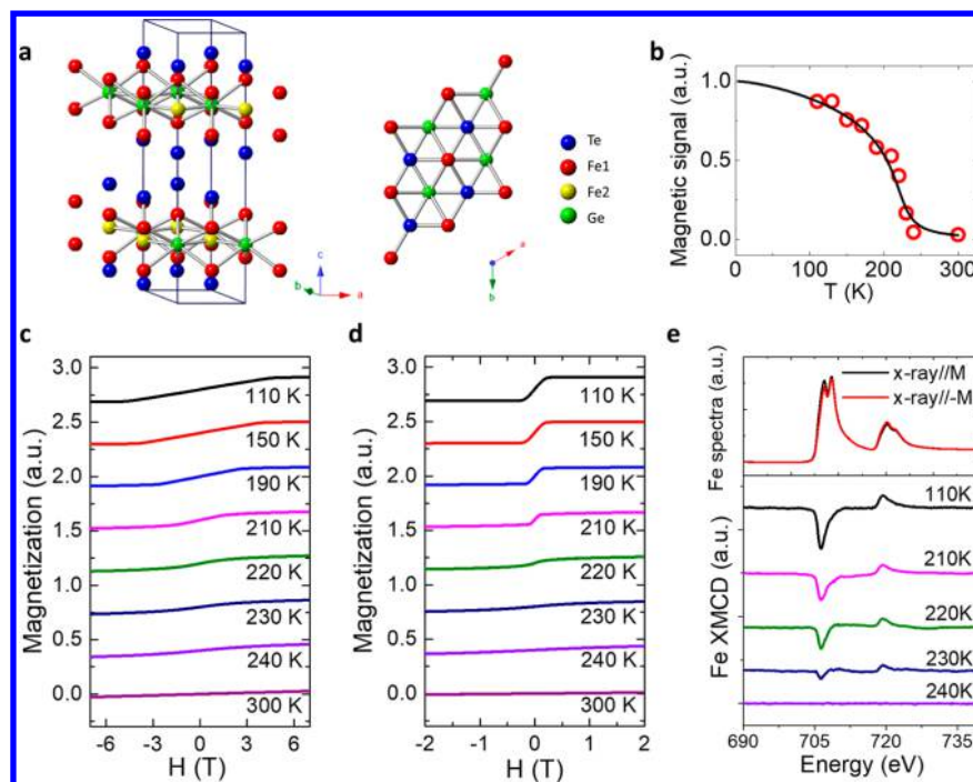
Figure 1. Crystal structure and magnetic measurement of \text{Fe}_3\text{GeTe}_2 . (a) Crystal structure (side view and top view) of \text{Fe}_3\text{GeTe}_2 . (b) Temperature dependence of the bulk \text{Fe}_3\text{GeTe}_2 magnetization (black line) measured using SQUID in a 0.7 T magnetic field along the magnetization easy axis ( c axis) after zero-field cooling. The red circles represent the Fe XMCD signal. Magnetic hysteresis loops measured with SQUID in magnetic fields applied (c) perpendicular to and (d) parallel to the c axis of bulk \text{Fe}_3\text{GeTe}_2 crystal at different temperatures. (e) Fe 2p level X-ray absorption spectra (XAS) at T = 110 K for magnetization parallel (black line) and antiparallel (red line) to the incident X-rays. The difference of the XAS (XMCD signal) measures the \text{Fe}_3\text{GeTe}_2 magnetic long-range order. Both SQUID and XMCD data show T_C \approx 230 K for bulk \text{Fe}_3\text{GeTe}_2 .
